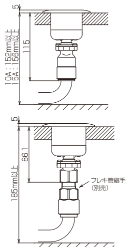
G855AC5-09P(10A, 15A)
