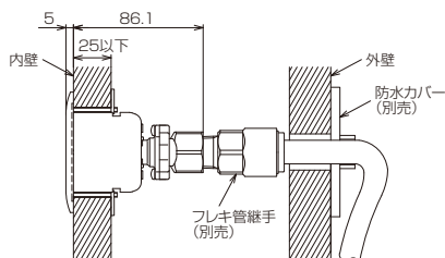
G858AC-09P(Rc1/2)
